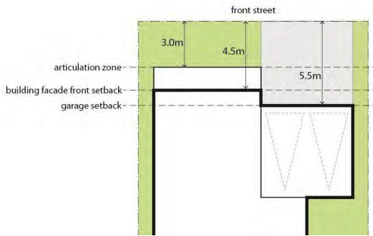
Figure 432: Minimum Front Setback Distances
