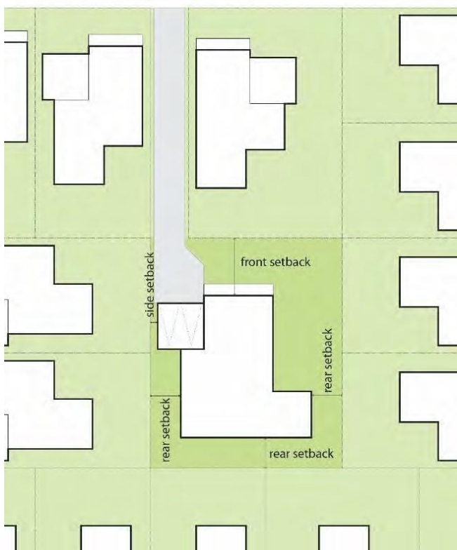
Figure 5346: Battle-axe Lot (Without any Street Frontage) Example of Setbacks
