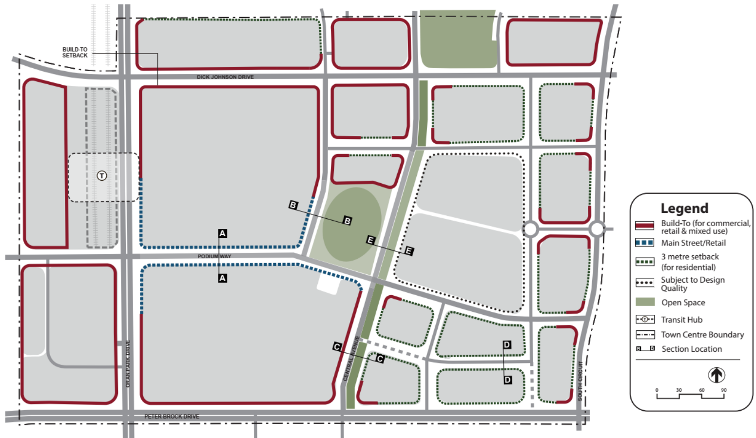
Figure 7279: Indicative "Build-To" Lines and Setbacks
