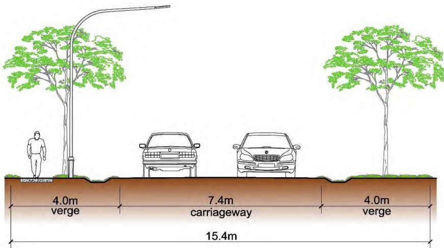
Figure 7: Ridgeline Interface Road Cross Section
