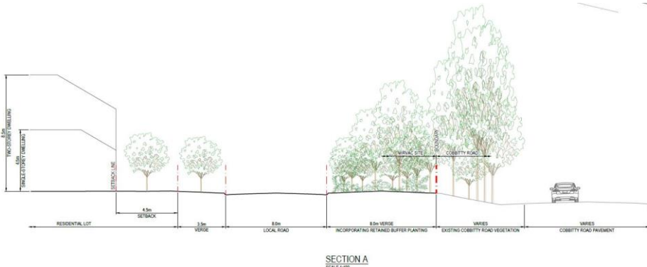
Figure 28: Cross Section of perimeter road which runs parallel with Cobbitty Road ( recommended post-exhibition amendment ).
