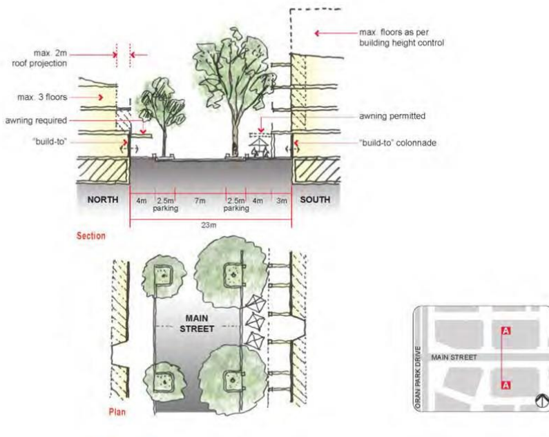
Figure 68-4: Section A – Main Street
