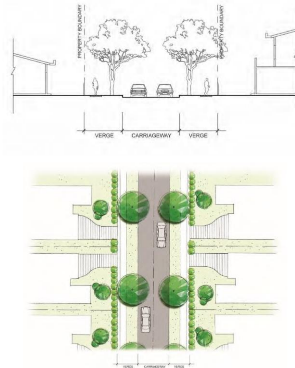
Figure 12: Indicative Layout of Local Street
