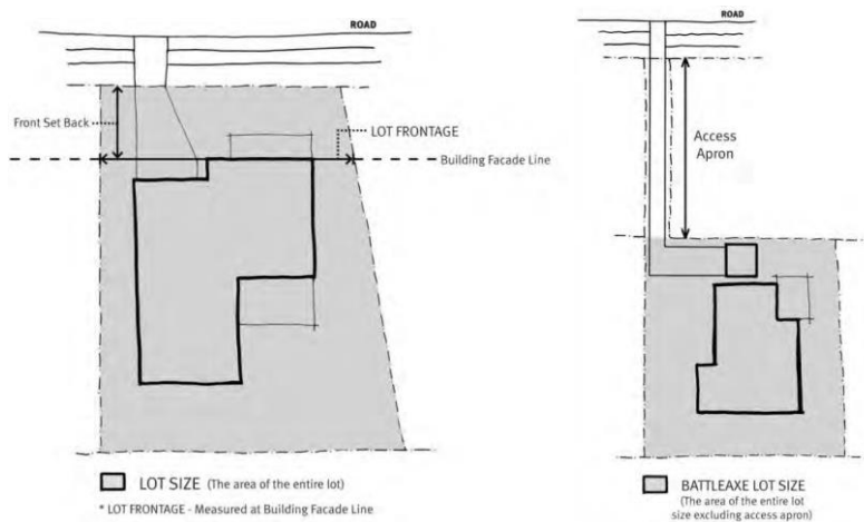
Figure 3239: Measurement of Minimum Lot Widths and Lot Area
