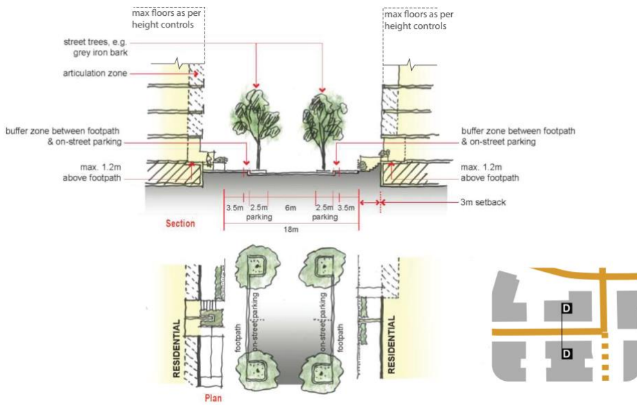
Figure 7063: Section D - Typical Secondary Street
