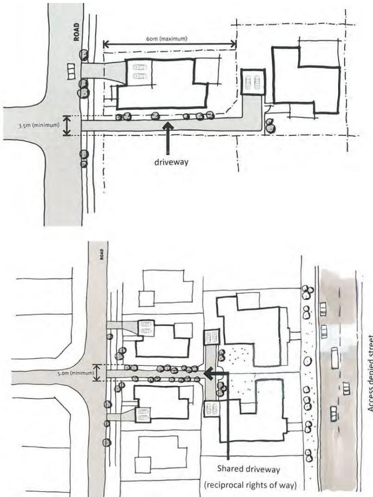
Figure 3542: Examples of Driveways and Shared Driveways for Battle-axe Lots
