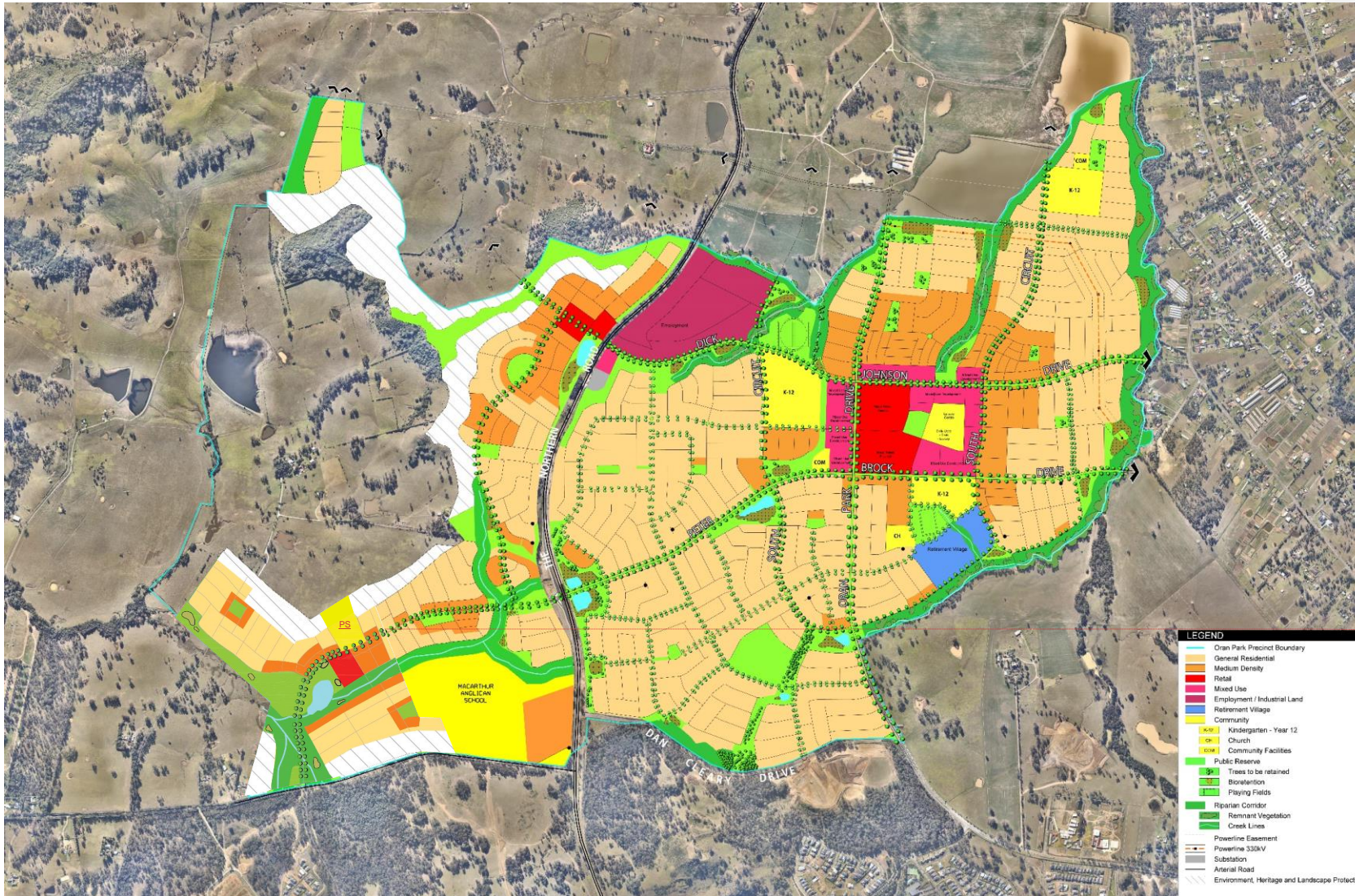
Figure 2: Oran Park Precinct Indicative Layout Plan (as amended in relation to amendment no.13)
