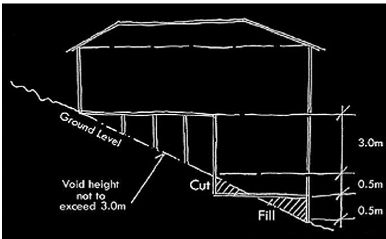
Figure 3946: Maximum Height of Voids Within Residential Lots
