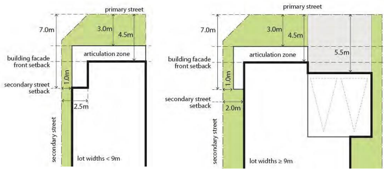
Figure 4451: Minimum Setbacks on Corner Lot Dwellings
