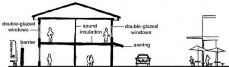
Figure 4956: Strategies for Minimising Noise Transmission
