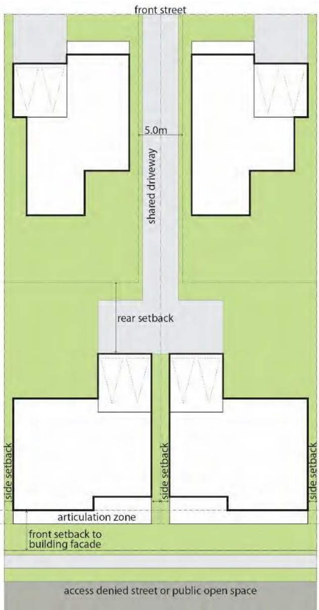
Figure 4754: Battle-axe Lot (Fronting Access Denied Road) Setbacks
