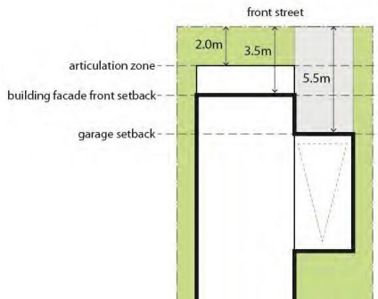
Figure 4350: Minimum Front Setbacks for Dwellings Fronting Open Space or Drainage Land
