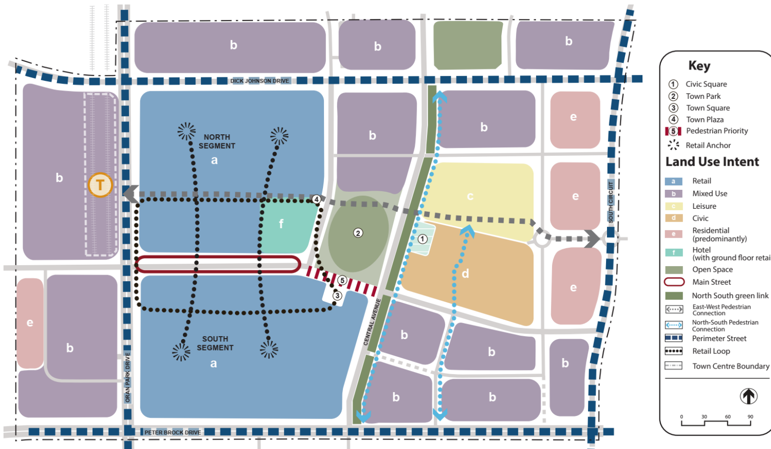
Figure 5057: Town Centre Structure Plan
